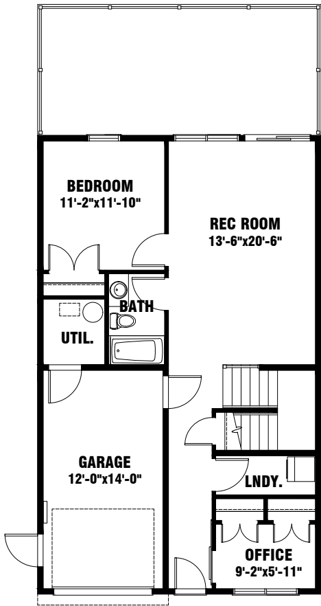
BASEMENT FLR.
