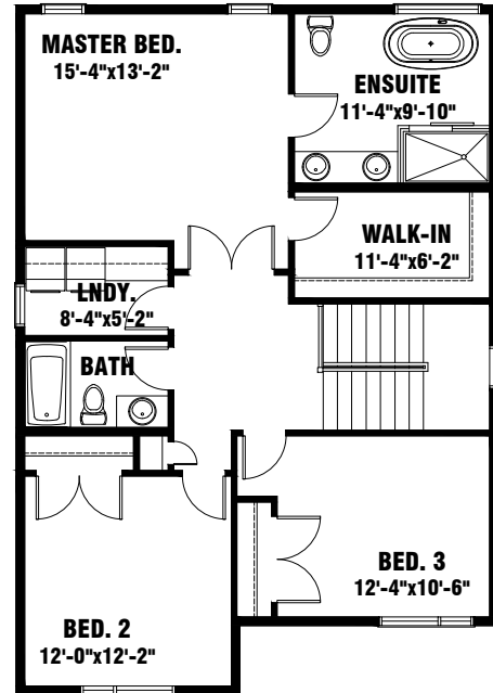
SECOND FLR.
