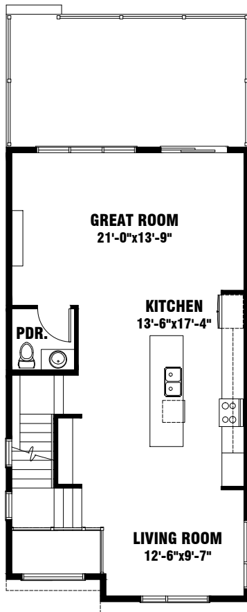
FIRST FLR.
