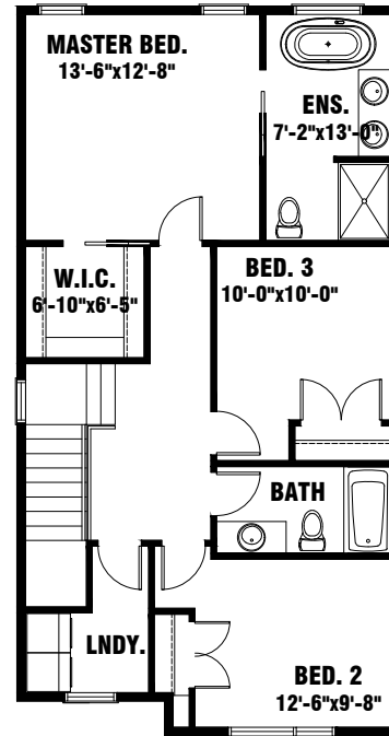
SECOND FLR.
