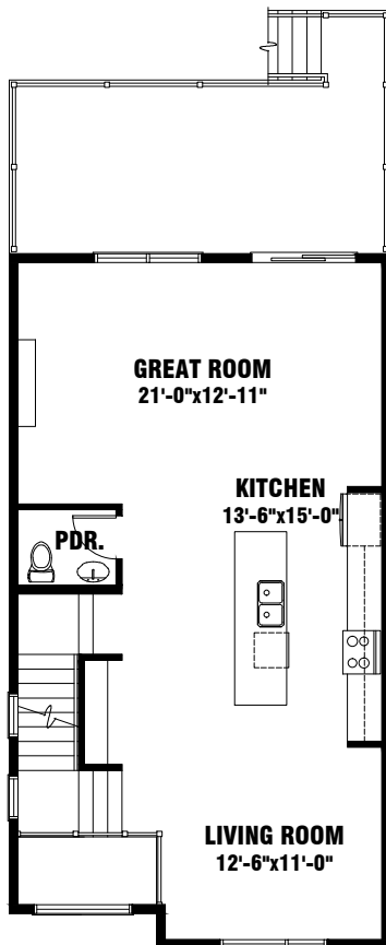
FIRST FLR.
