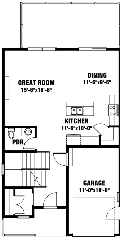
FIRST FLR.
