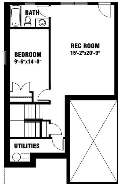
BASEMENT FLR.
